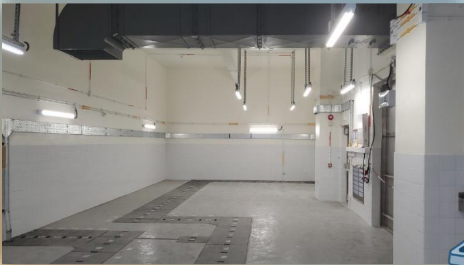
Completed Building Services installation at Transformer Room 變壓房屋宇裝備工程完成
